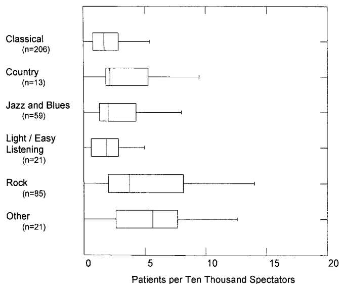
Figure 1. Numbers of patients compared by type of concert. In the boxplots shown, the center vertical line is the median of each sample, with the box edges marking the interquartile range. The lines on either side represent the range of values that fall within 95% confidence intervals.
